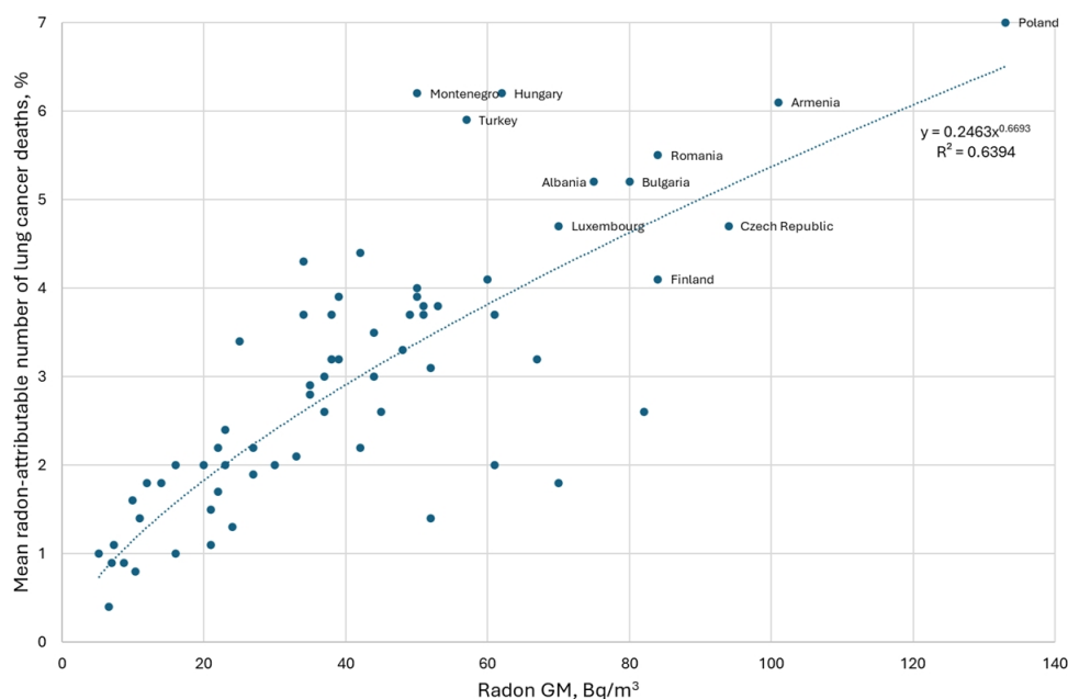
Fig. 1. Average number of lung cancer deaths attributable to radon (vertical axis, %) and average radon concentrations in buildings (horizontal axis, Bq/m 3 ), source: Bobkier, R., Kovler, K., Tsapalov, A., 2025. "Fusion of Horizons": Part I. Historical context and early radon discoveries (until 1951). Journal of Environmental Radioactivity , No. 283, p. 3.
